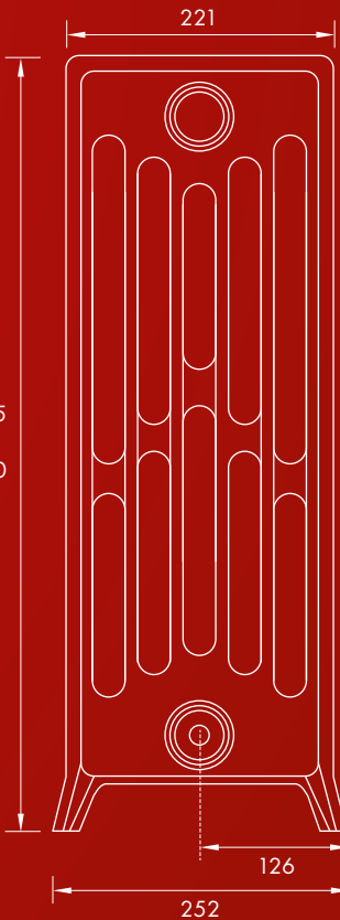
Stelrad Hattersley Cast Iron Column 6
