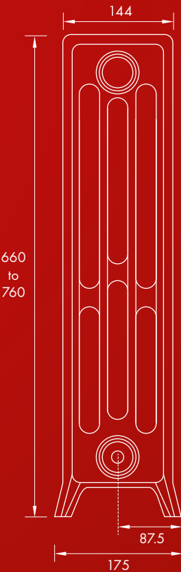
Side View - Stelrad Hattersley Cast Iron Column 4
