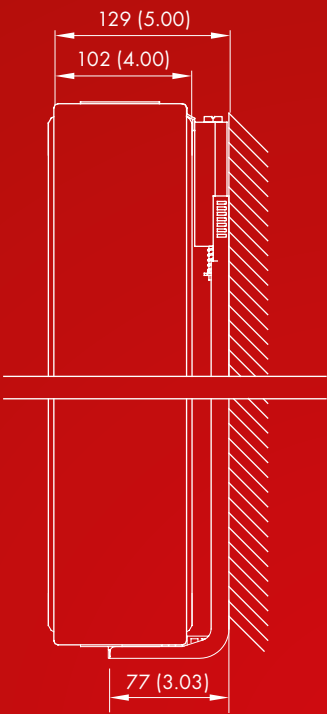
Side View - Vertical Panel T22
