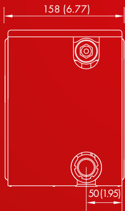
Type 33 (200mm high)
