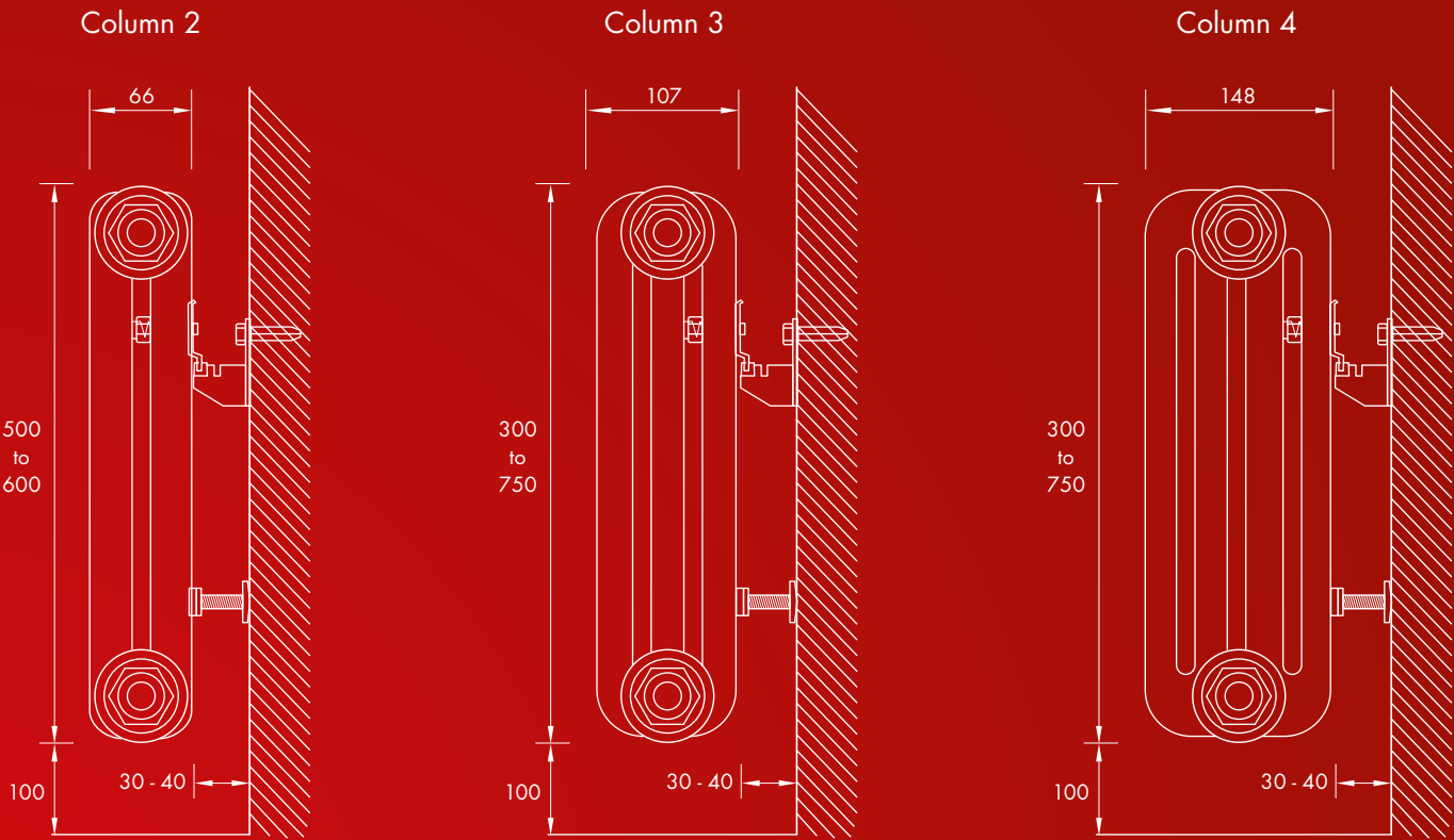
Side View - Column Horizontal
