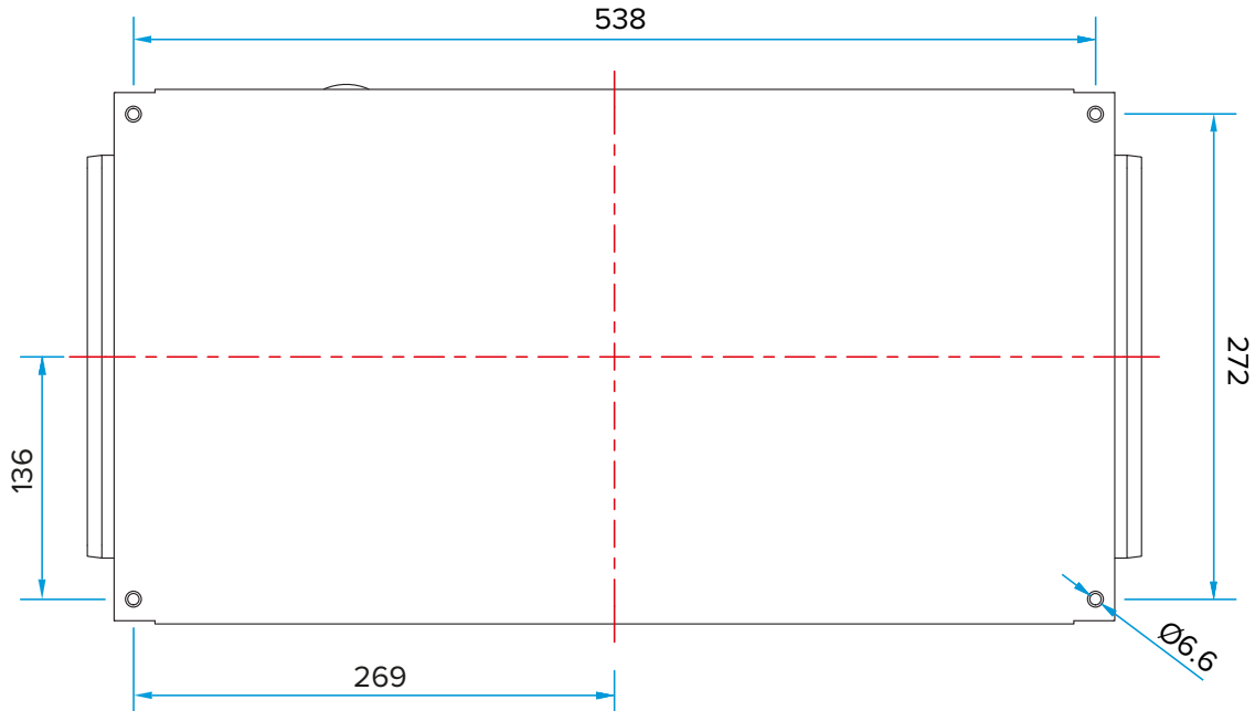
Fig 2: Mounting Hole Dimensions (mm)
