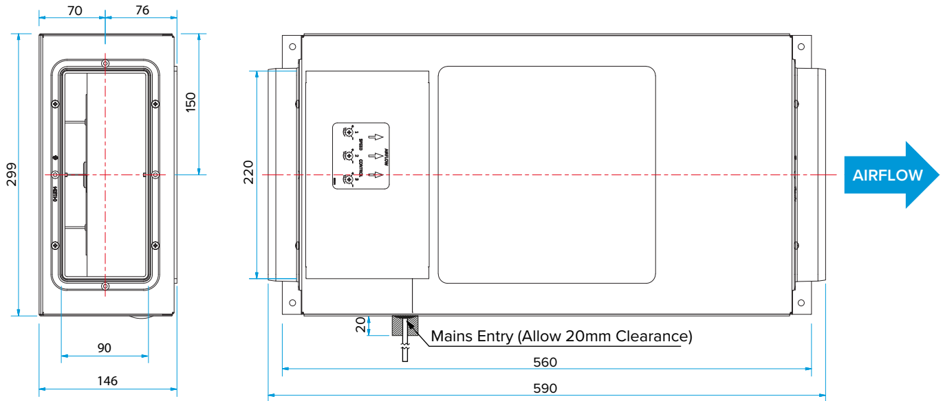
Fig 1: Unit Dimensions (mm)
