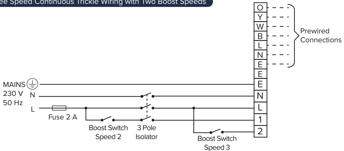
Fig 7: Three Speed Continuous Trickle Wiring with Two Boost Speeds
